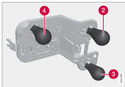
Taillight bulb holder
