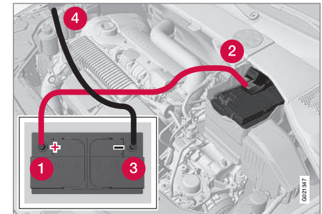
Connecting the jumper cables
