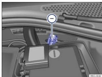
Fig. 168 In the engine compartment: Negative jump-start terminal ⊖.
