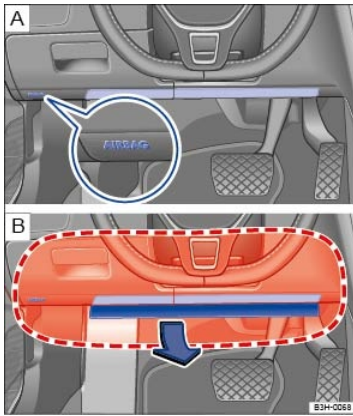
Fig. 42 On the driver side: Location and deployment zone of the knee airbag.
