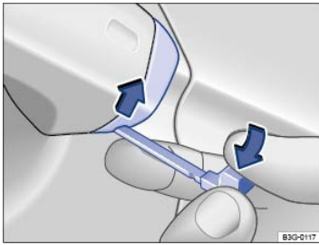
Fig. 66 Driver door handle: Removing the lock cylinder cover.
