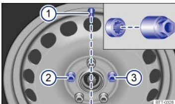
Fig. 196 Changing a wheel: Tire valve ① and installation points for the anti-theft wheel bolt (if equipped) ② or ③.
