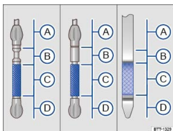
Fig. 178 Engine oil dipstick with oil level marks.
