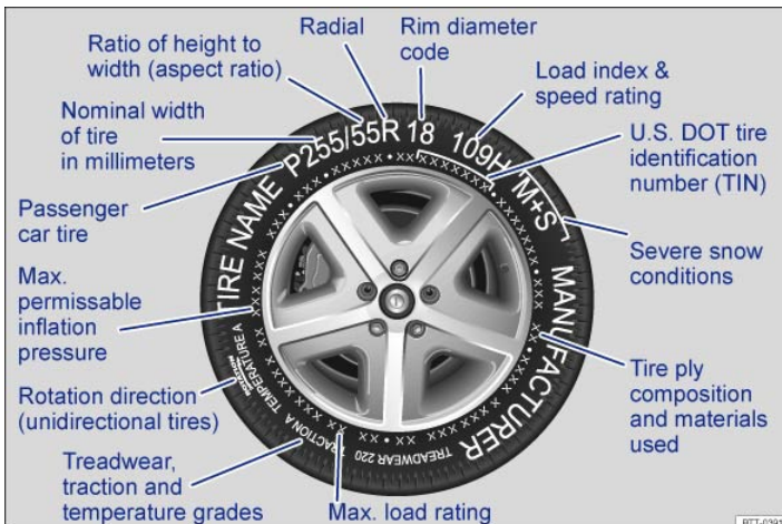
Fig. 190 International tire labeling.
