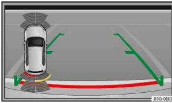
Fig. 127 Mini PDC display of the area around the vehicle (display may vary depending on vehicle equipment).
