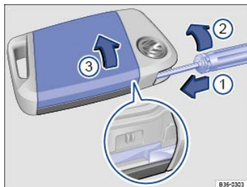
Fig. 57 Remote control vehicle key: Opening the battery compartment cover.
