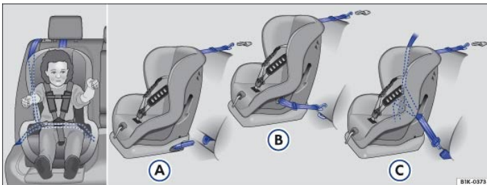
Fig. 47 All convertible child restraints have lower anchors and a top tether. Figures A and B show how to correctly install a LATCH/UCRA seat. Figure C shows the set up of a seat using the vehicle's safety belt system.
