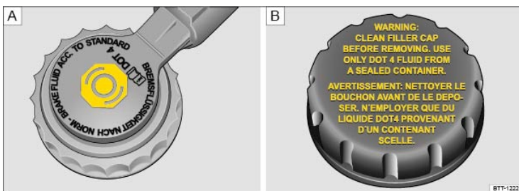
Fig. 182 In the engine compartment: Brake fluid reservoir cap (cap design may vary depending on vehicle equipment).
