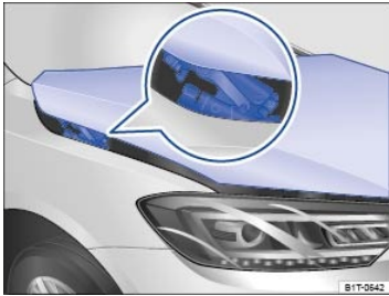
Fig. 54 Re-active hood after it has been triggered.
