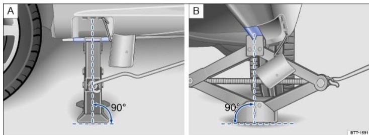
Fig. 199 Jack in position at the left rear lift point.
