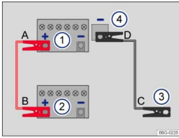
Fig. 169 Diagram for attaching the jumper cables: Dead battery ① and booster battery ②.
