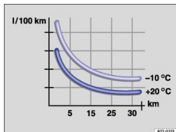
Fig. 104 Fuel consumption in l/100 km at two different outside air temperatures.
